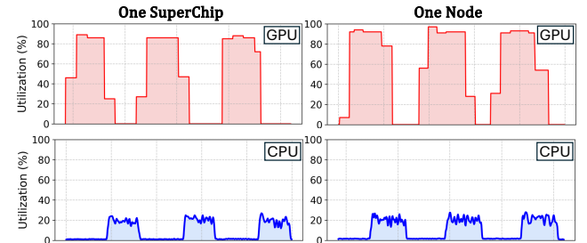
Figure 4. Prior offloading-based solutions cause idle time on both GPU and CPU side. We evaluate it using the largest model size that offloading-based solutions (ZeRO-Offload) can accommodate, along with the maximum batch size that prevents out-of-memory errors, on single Superchip and one node. The results show that during each training iteration, the GPU remains idle for 40-50% of the total execution time.
