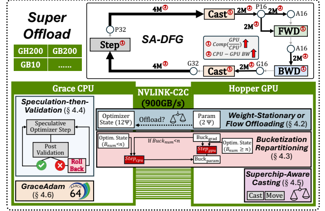
Figure 5. Overview of SuperOffload. At a high level, SuperOffload employs a Superchip-centric design that judiciously optimizes data placement, computation, and tensor migration between the Hopper GPU and Grace CPU, while fully utilizing the NVLink-C2C via a combination of techniques.
