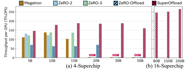
Figure 11. Training throughput comparison between Megatron, ZeRO-2/3, ZeRO-Offload, and SuperOffload on 4 and 16 GH200 GPUs. We use batch sizes of 16 and 128 for the 4-GPU and 16-GPU experiments, respectively.
