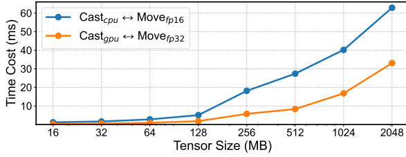
Figure 9. Time cost comparison for casting operations on GPU vs. CPU (including data transfer overhead).
