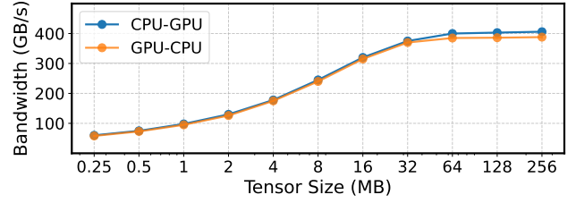
Figure 7. GH200 bandwidth measurement.
