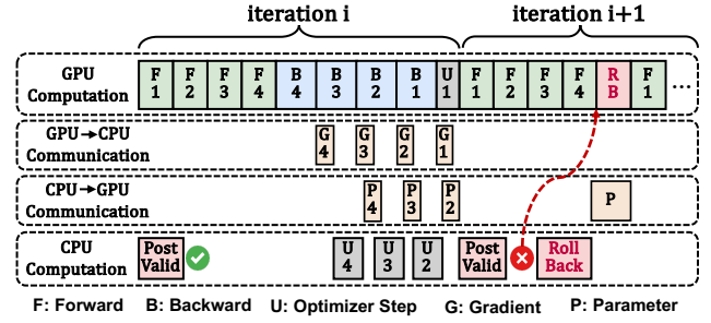
Figure 8. SuperOffload speculation-then-validation schedule. It enables optimizer steps (U) to overlap with backward propagation (B), eliminating synchronization bottlenecks and improving resource utilization.
