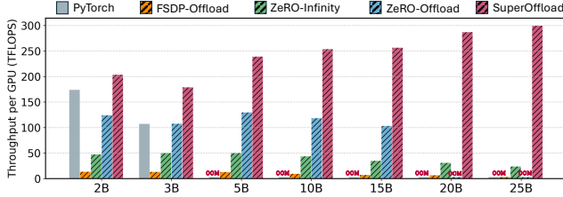
Figure 10. The training throughput with PyTorch DDP, FSDP-Offload, ZeRO-Infinity, ZeRO-Offload, and SuperOffload on a single Superchip with batch size 8.
