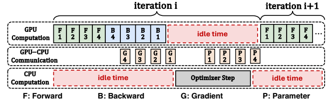
Figure 3. ZeRO-Offload computation idle time on both GPU and CPU side.
