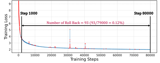
Figure 14. Training loss and rollback occurrences during training of the GPT 176B model over 80,000 iterations. Red dots indicate iterations where rollbacks were triggered due to gradient clipping, NaN or INF values.
