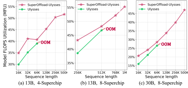
Figure 12. Supported sequence lengths and corresponding MFU using SuperOffload-Ulysses and Ulysses. OOM denotes the point where increasing sequence length causes OOM.
